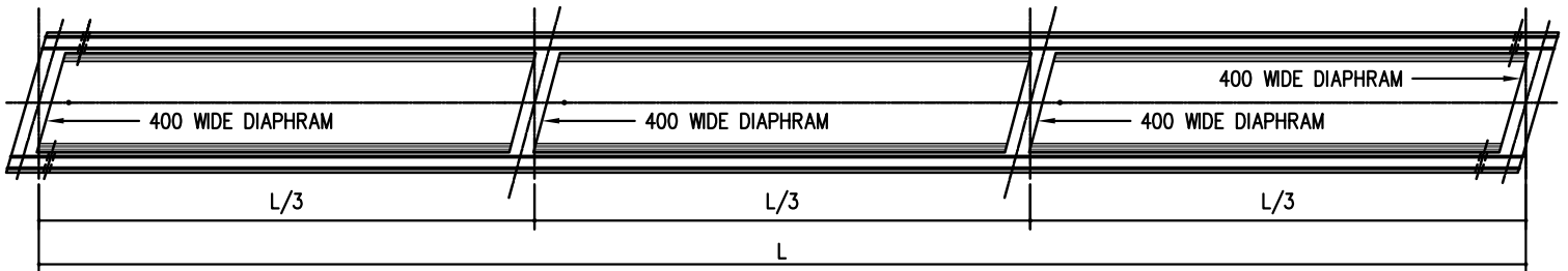
TYPICAL PLAN OF SPECIAL U BEAM
